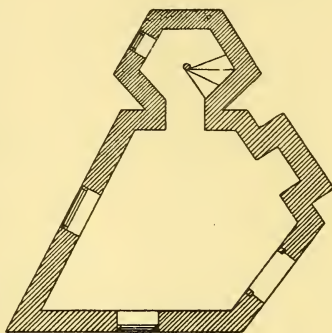
10 5 0 10 PLAN OF GARDEN HOUSE AT AMESBURY.
